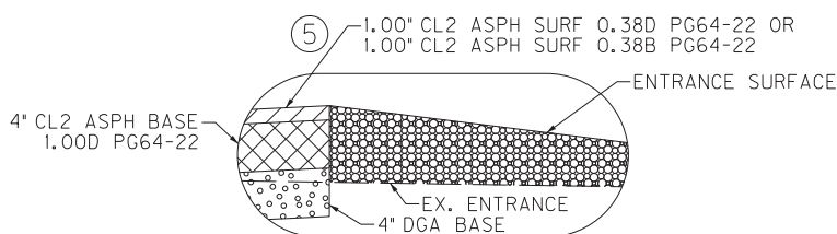
ENTRANCE DETAIL
