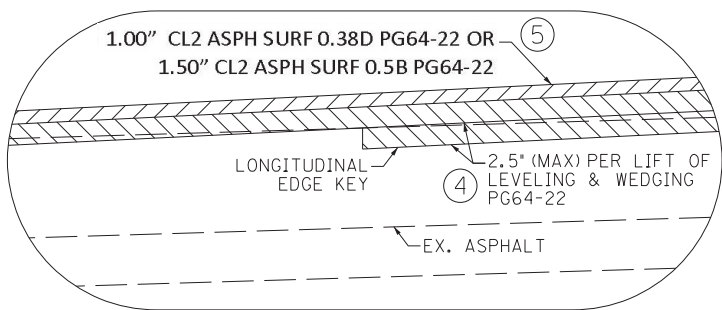
DETAIL "B"
